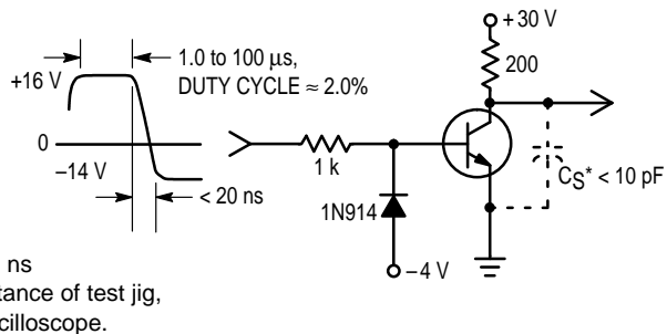
Figure 2. Turn-Off Time
