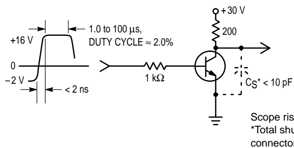
Figure 1. Turn-On Time
